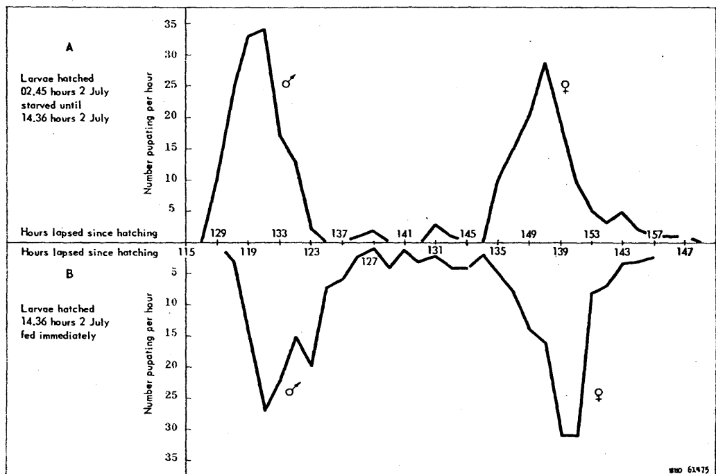
EFFECT OF STARVATION OF FIRST-STAGE LARVAE OF C. P. FATIGANS ON DURATION OF LARVAL LIFE
