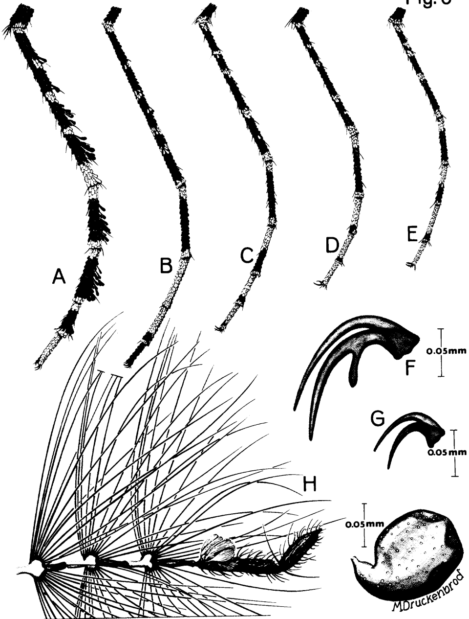
Figure.6 Aedeomyia (L.) fufurea , A, ♀ hind tarsus; F, ♂ fore tarsal claw; H, apical flagellomeres of ♂ antenna. Aedeo.(A.) venustipes , B, ♀ hind tarsus. Aedeo.(A.) squamipennis , C, ♀ hind tarsus. Aedeo.(A.) catasticta , D, ♀ hind tarsus; G, ♀ hind tarsal claw; I, spermatheca. Aedeo.(A.) africana , E, ♀ hind tarsus
