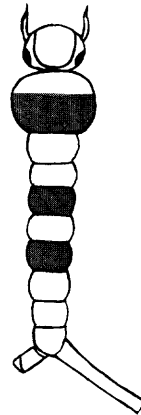
Cx. poecilipes
